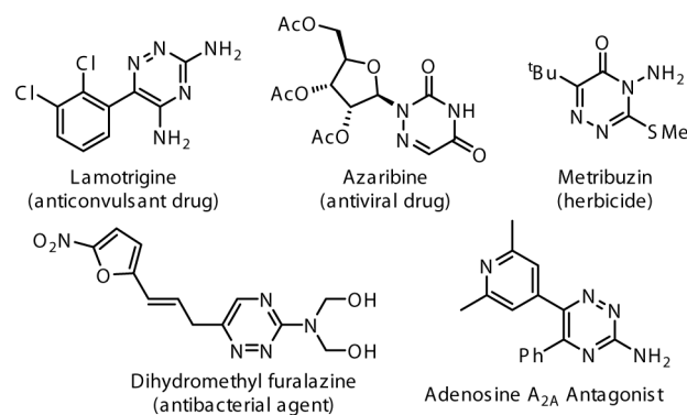
Figure 2. Selected biologically active 1,2,4-triazines.
