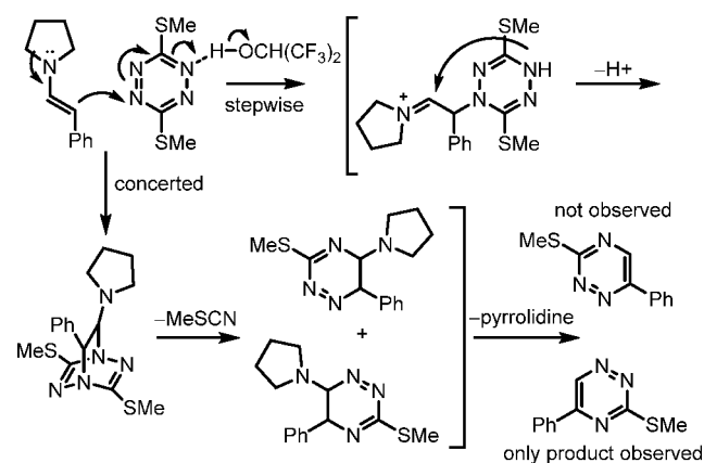
Figure 7. Plausible but improbable mechanisms.
