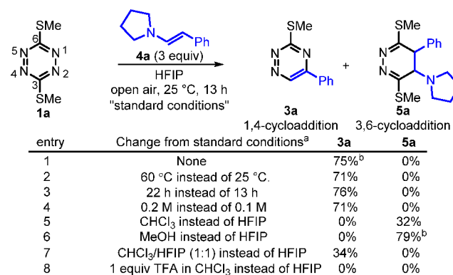
Figure 3. Reaction parameters. a Unless otherwise noted, all the reactions were run with 1a (0.05 mmol) in 0.5 mL solvent. b Isolated yield, other yields were established by NMR.
