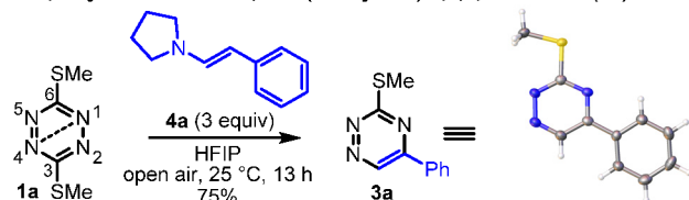
Figure 1. Cycloadditions of 1,2,4,5-tetrazines (C3/C6 cycloaddition) and the unprecedented formal 1,4-cycloaddition (N1/N4) detailed herein.
