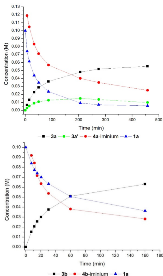
Figure 9. Reaction profile over time for reaction of 1a with 4a (top) and 4b (bottom).
