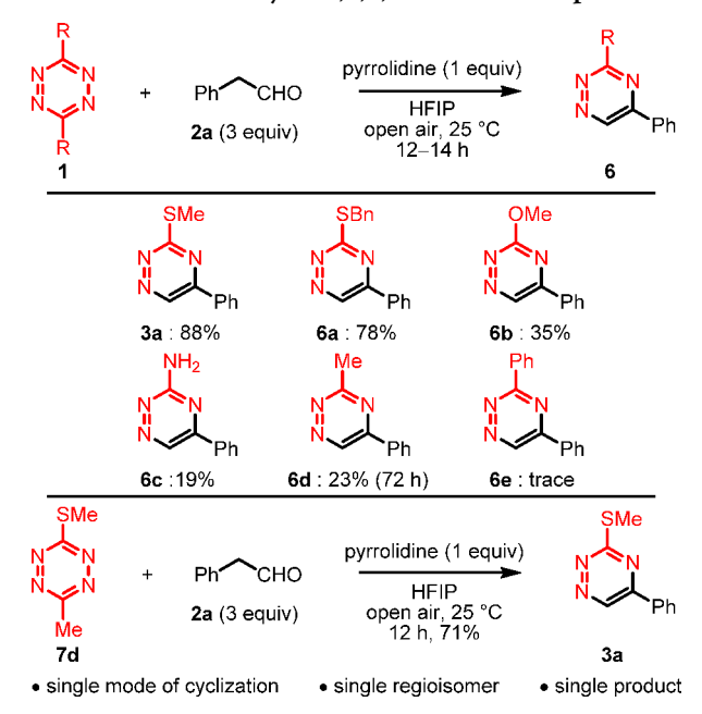
Figure 6. Reaction of unsymmetrical 1,2,4,5-tetrazines. a Yield established by NMR. Others are isolated yields.
