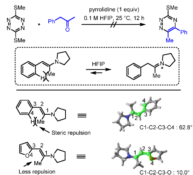
Figure 5. Steric repulsion of the pyrrolidine enamine of 1-phenylacetone versus the in situ generated enamine of 2p.
