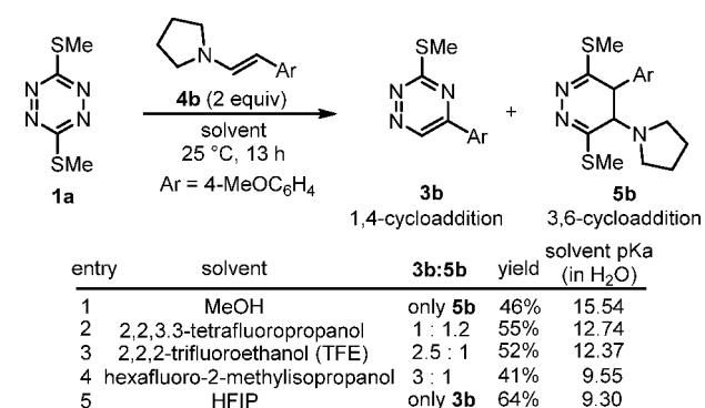
Figure 4. Refined solvent survey. Yields were established by NMR.
