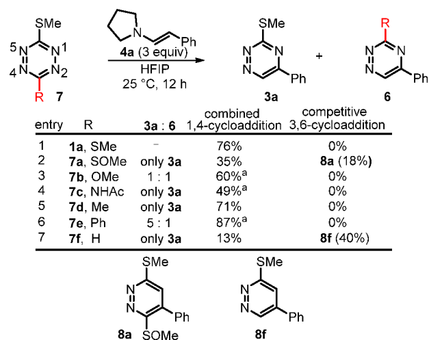
Figure 6. Reaction of unsymmetrical 1,2,4,5-tetrazines. a Yield established by NMR. Others are isolated yields.
