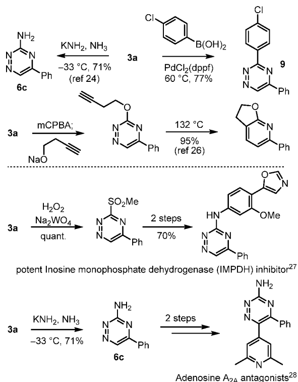
Figure 12. Representative diversification of 3a and its use in the synthesis of biologically active compounds.
