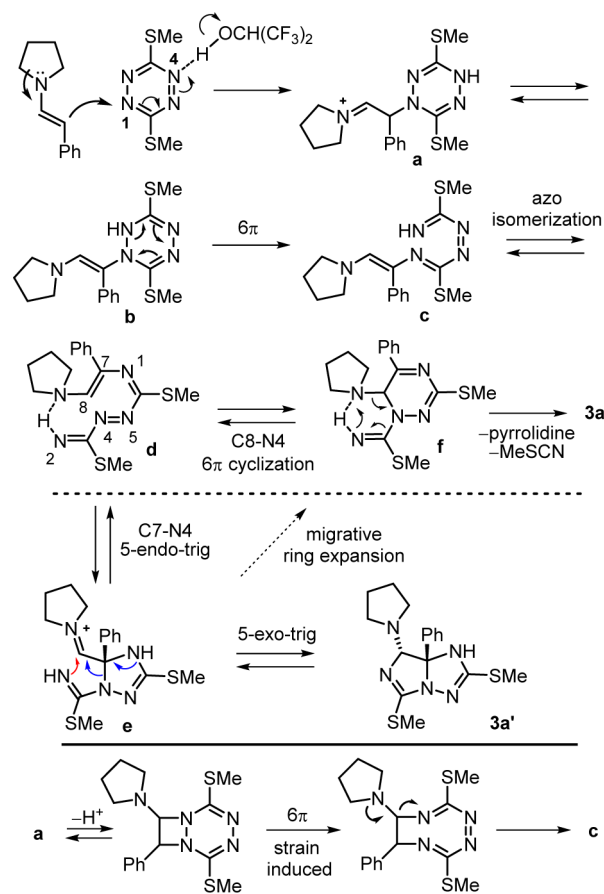
Figure 11. Plausible reaction pathway.
