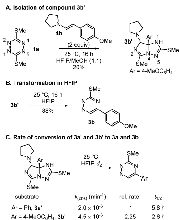
Figure 10. Related studies of compound 3b' .
