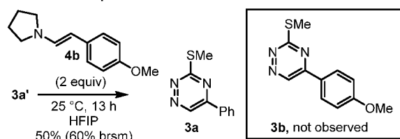
Figure 8. Isolation and studies of compound 3a'.
