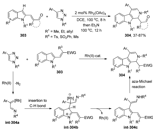
Scheme 94 Rh(III)-catalyzed carbene insertion/[4+3] annulation of 2-vinylindoles with N -sulfonyl-1,2,3-triazoles.
