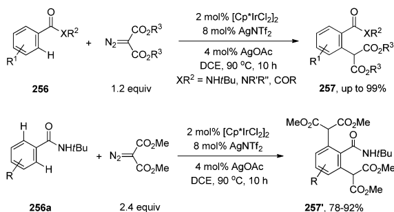
Scheme 80 Ir(III)-catalyzed aryl C(sp 2 )-H functionalization by carbene insertion with diazo compounds.
