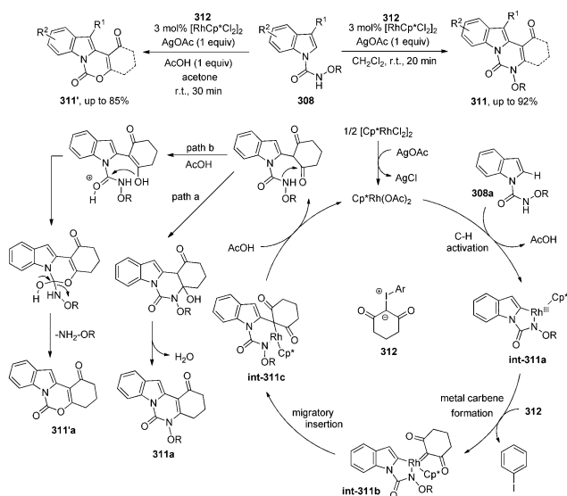
Scheme 96 Rh(III)-catalyzed, acid-controlled chemodivergent annulations between indoles and iodonium carbenes.
