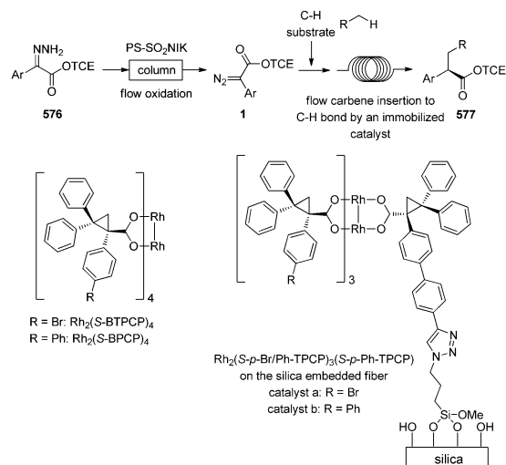
Scheme 146 The hollow fiber reactor strategy for chiral Rh(II)-catalyzed carbene insertion to C(sp 3 )-H bonds with diazo compounds.
