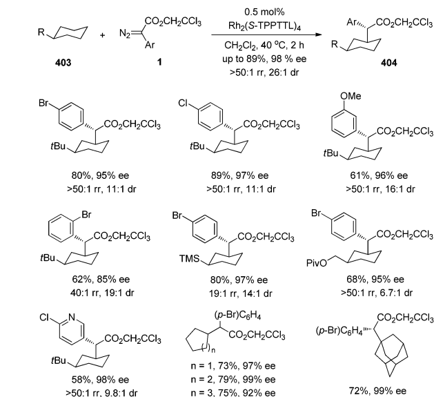
Scheme 120 Rh(II)-catalyzed site- and enantioselective C–H functionalization of non-activated cycloalkanes by carbene insertion.
