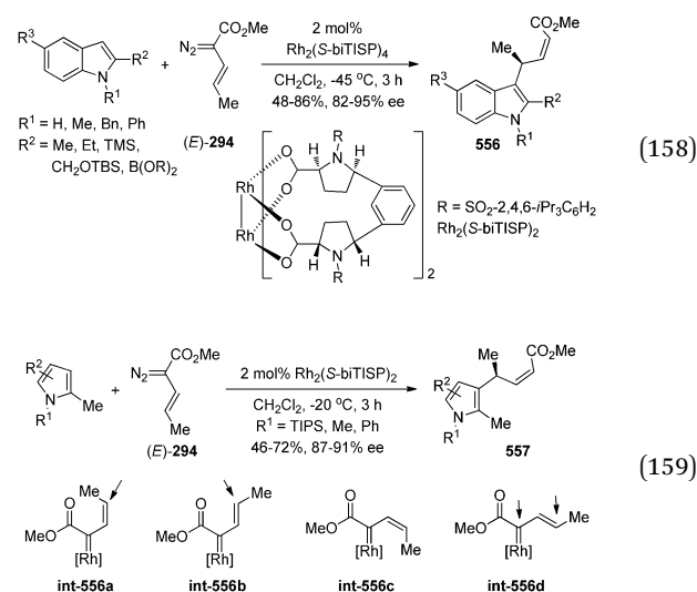
Scheme 141 Rh(II)-catalyzed enantioselective carbene insertion to indolyl C(sp 2 )-H bonds.
