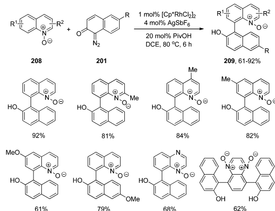
Scheme 66 Rh(III)-catalyzed C(8)-arylation of quinoline N -oxides.
