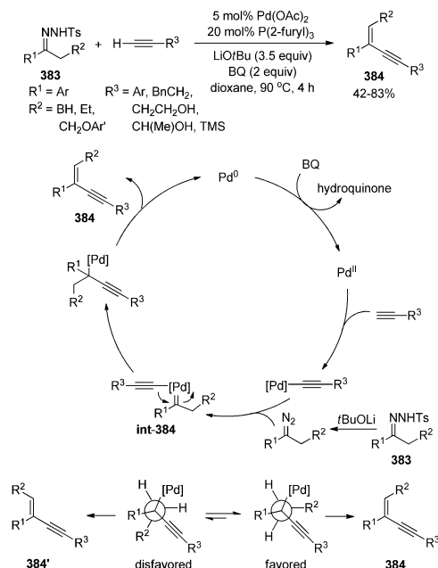
Scheme 113 Palladium-catalyzed oxidative cross-coupling of terminal alkynes with N -tosylhydrazones.
