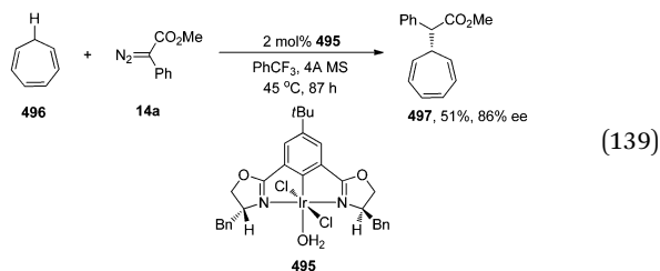
Scheme 131 Rh(II)-catalyzed formal enantioselective intermolecular carbene insertion to allylic \text{C}(\text{sp}^3)\text{--H} bond.
