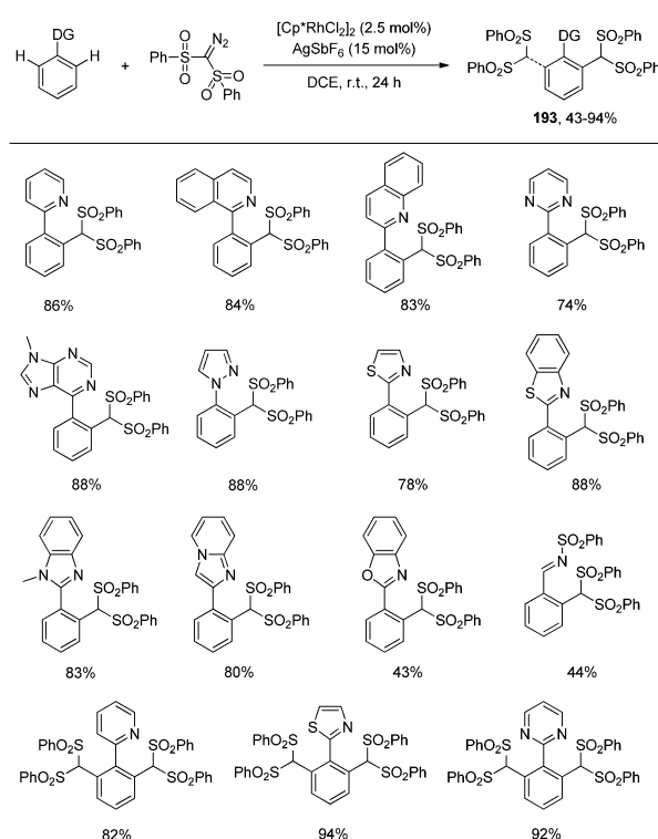
Scheme 63 Rh(III)-catalyzed, N-heteroaryl-directed C–H functionalization of aryl C(sp 2 )–H bonds with bis(phenylsulfonyl)diazomethane.
