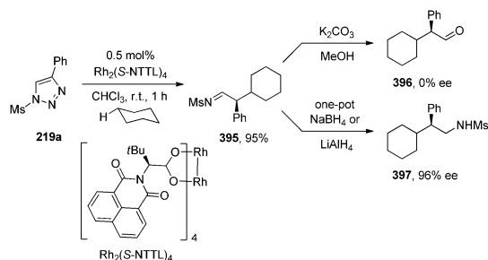
Scheme 116 Rh(II)-catalyzed enantioselective azavinyl carbene insertion to cyclohexane C–H bond.
