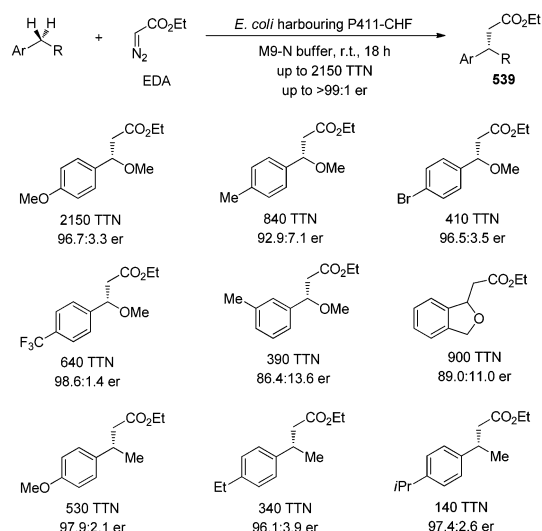
Scheme 137 Enzymatic carbene insertion to benzylic C–H bonds.
