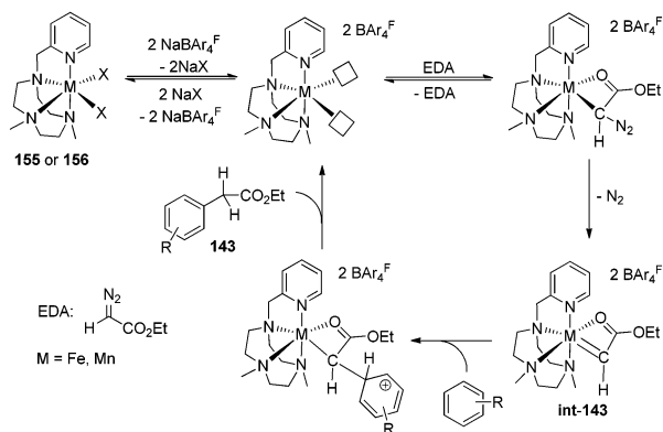
Scheme 55 Proposed mechanism for Fe–N 4 and Mn–N 4 catalyzed C–H functionalization of non-activated arene by carbene insertion with EDA.
