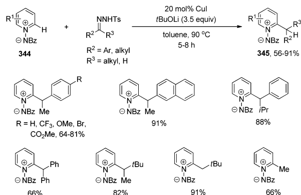
Scheme 102 Cu(I)-catalyzed carbene insertion to C(2)-H bond of N -iminopyridinium ylides.
