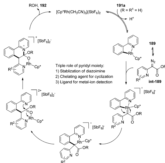
Scheme 62 Rh(III)-catalyzed, 2-pyridyl-directed C–H functionalization of aryl C(sp 2 )–H bond.
