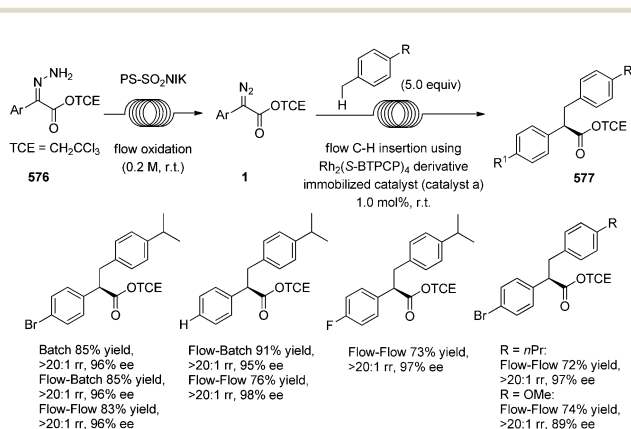
Scheme 147 Chiral Rh(II)-catalyzed flow carbene insertion to C(sp 3 )-H bonds with diazo compounds in a hollow fiber reactor.
