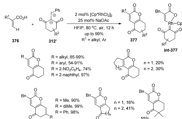
Scheme 110 Rh(III)-catalyzed formal carbene insertion to alkenyl C–H bonds with iodonium ylides.
