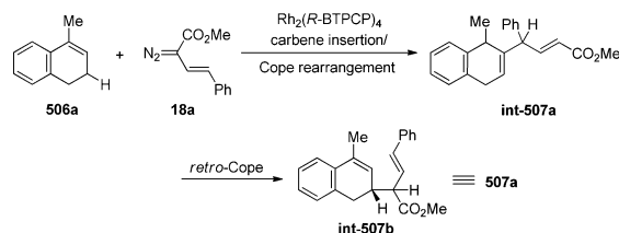
Scheme 131 Rh(II)-catalyzed formal enantioselective intermolecular carbene insertion to allylic \text{C}(\text{sp}^3)\text{--H} bond.
