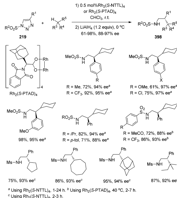
Scheme 117 Rh(II)-catalyzed enantioselective direct C–H functionalization of non-activated alkanes.
