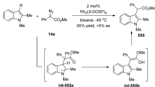
Scheme 140 Rh(II)-catalyzed carbene insertion to indolyl C(sp 2 )-H bonds.
