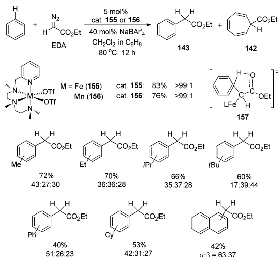
Scheme 54 Fe–N 4 and Mn–N 4 catalyzed C–H functionalization of non-activated arene by carbene insertion with EDA.
