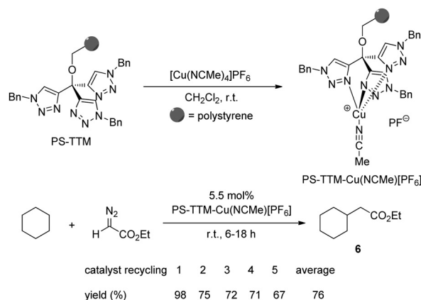
Scheme 12 PS-TTM- \text{Cu}(\text{NCMe})[\text{PF}_6] -catalyzed carbene insertion to the C–H bond of cyclohexane.
