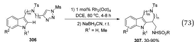
Scheme 94 Rh(III)-catalyzed carbene insertion/[4+3] annulation of 2-vinylindoles with N -sulfonyl-1,2,3-triazoles.
