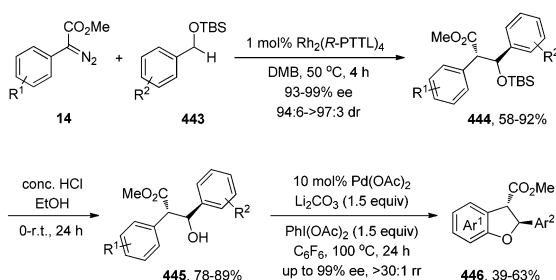
Scheme 127 Rh(II)-catalyzed enantioselective intramolecular carbene insertion to silyloxy-adjacent \text{C}(\text{sp}^3) –H bonds.
