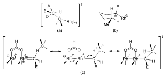
Scheme 18 Transition state models of C–H functionalization with diazo compounds and Rh 2 L 4 . (a) Doyle's 3e-center model. 4 (b) Taber's model. 135 (c) One metal center-dominating model. 134
