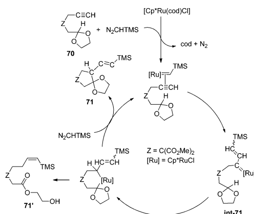
Scheme 33 Ru(II)-catalyzed 1,5-H/1,6-H shift cyclization sequence in alkynyl acetals and ethers with N 2 CHTMS.
