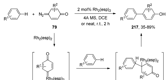
Scheme 68 Rh(II)-catalyzed aryl C(sp 2 )-H functionalization by carbene insertion.
