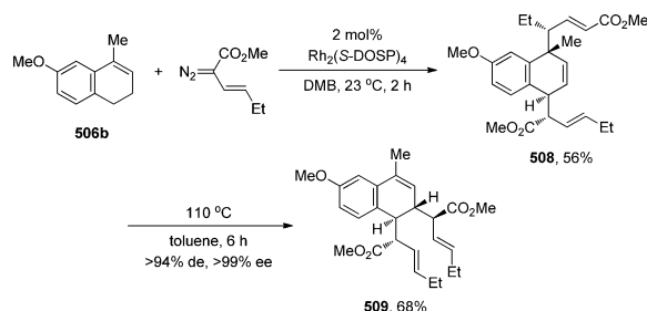
Scheme 132 Rh(II)-catalyzed enantioselective intermolecular double carbene insertion to allylic and benzylic \text{C}(\text{sp}^3)\text{--H} bonds.
