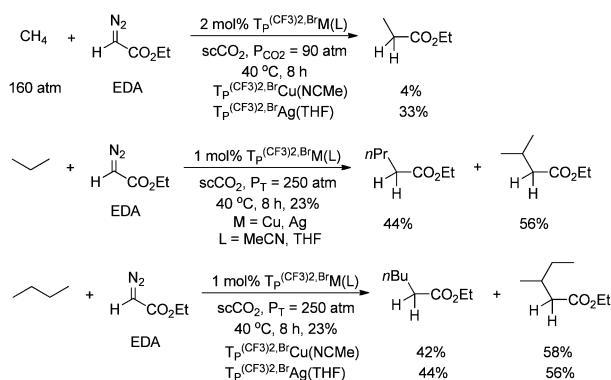
Scheme 15 C–H functionalization of propane and butane with EDA and \text{Tp}^{(\text{CF}_3)_2, \text{Br}}\text{M} -based catalysts (M = Cu, Ag). P_T = total pressure.
