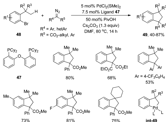
Scheme 26 Pd(II)-catalyzed intermolecular carbene insertion to alkyl C–H bonds.
