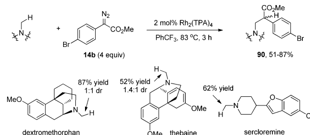
Scheme 35 \text{Rh}(\text{II}) -catalyzed carbene insertion to primary C–H bonds of the N -CH 3 moiety in N -methyl-containing natural products and drug molecules.
