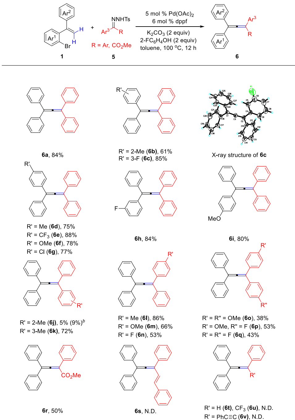
Scheme 3. Cross-Coupling of 1-Bromo-2-Vinylbenzenes ( 1 ) with N -Tosylhydrazones of Diaryl Ketones ( 5 ) a,b
