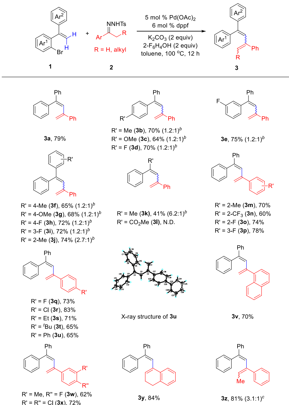
Scheme 2. Cross-Coupling of 1-Bromo-2-vinylbenzenes ( 1 ) with N -Tosylhydrazones of Aryl Alkyl Ketones ( 2 ) a,b,c
