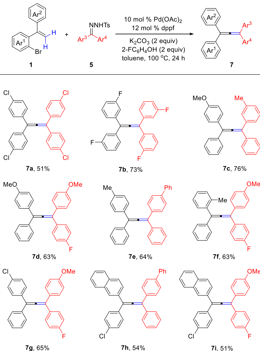
Scheme 4. Synthesis of Diverse Tetraaryl-Substituted Allenes (7) a
