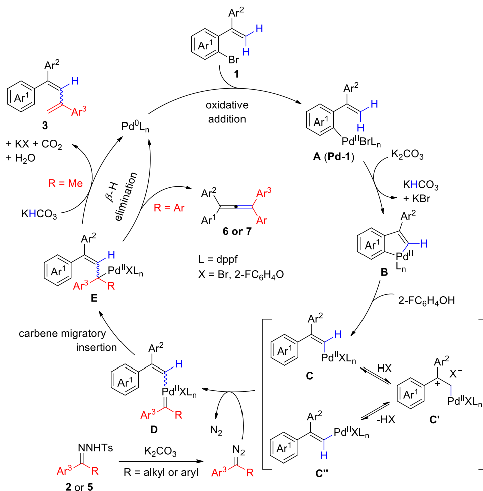
Scheme 8. Proposed Mechanism
