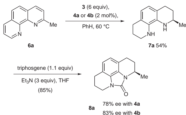
Scheme 2 Brønsted acid catalyzed asymmetric reduction of 2-methyl-1,10-phenanthroline.
