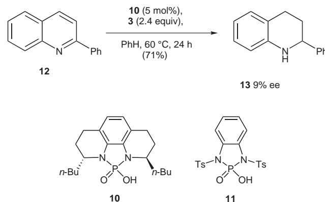
Scheme 3 Reduction of 2-phenylquinoline catalyzed by phosphorodiamidic acid 10 .
