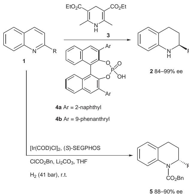
Scheme 1 Brønsted acid and iridium-catalyzed asymmetric reduction of quinolines.
