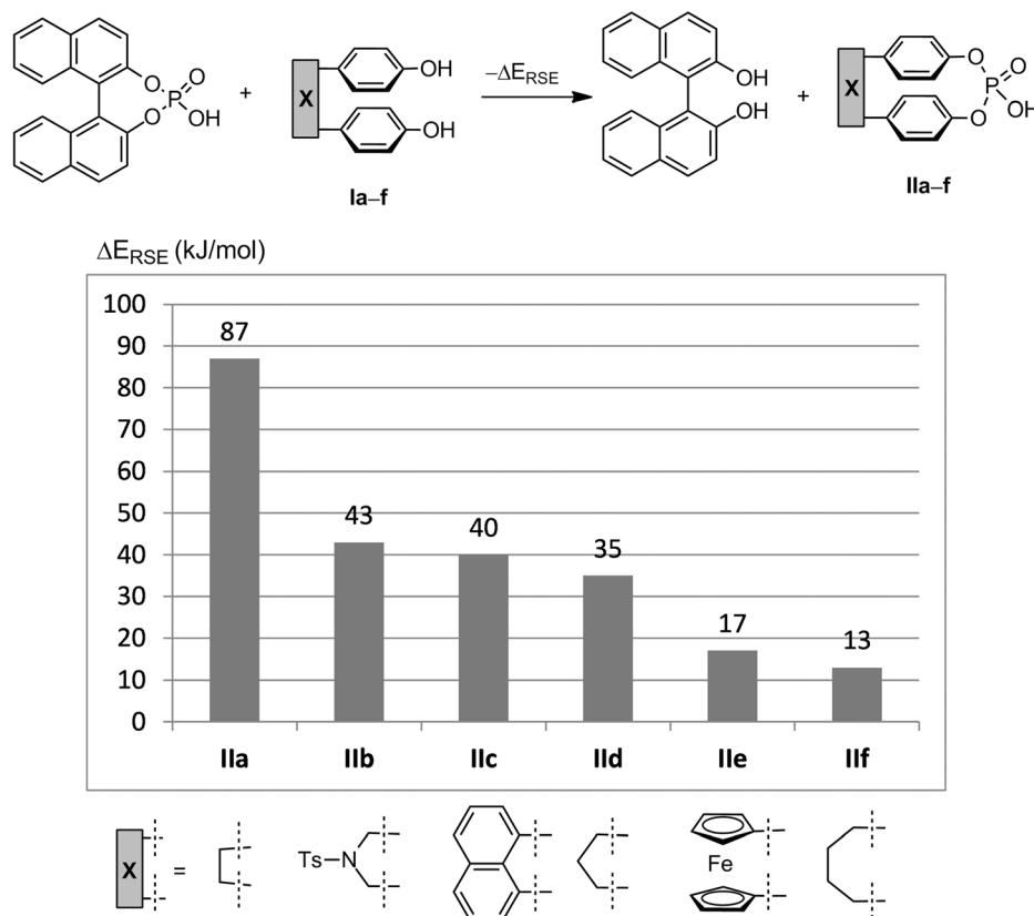
Scheme 1. Isodesmic reaction used to compute the relative ring strain energy of IIa–f relative to the BINOL-derived phosphoric acid.
