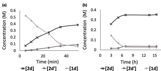
Figure 6. Time courses of the Pd-catalyzed C–N coupling reaction of p -chlorotoluene ( 1d ) and hydrazine with a) 5 mol% of Pd catalyst at 60 °C for 50 min; b) 800 ppm of Pd catalyst at 100 °C for 15.5 h.
