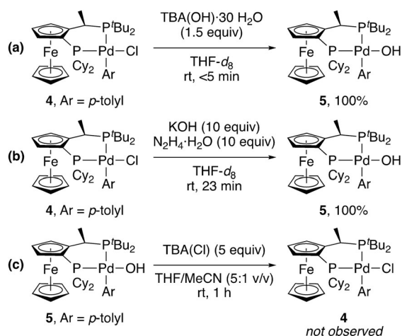
Scheme 4. Reactions of arylpalladium(II) chloride complex 4 with hydroxide sources and reactions of arylpalladium(II) hydroxide complex with TBA(Cl).
