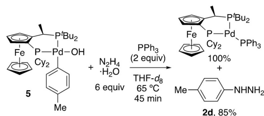
Scheme 3. Reaction of arylpalladium(II) hydroxide complex 5 with hydrazine.
