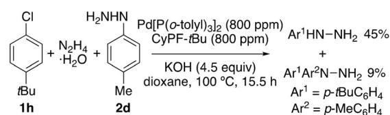
Scheme 5. Competition experiment between hydrazine and p -tolyl hydrazine under catalytic conditions.
