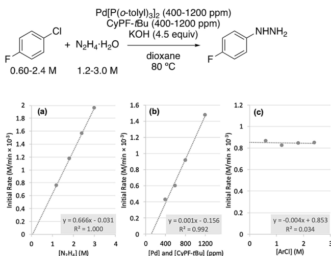
Figure 1. Kinetic studies on the monoarylation of hydrazine. a) Dependence of initial rate on [N 2 H 4 ] (1.2–3.0 M) with [ArCl] = 0.60 M and [Pd] and [CyPF- t Bu] = 800 ppm. b) Dependence of initial rate on [Pd] and [CyPF- t Bu] (400–1200 ppm) with [ArCl] = 0.60 M and [N 2 H 4 ] = 1.8 M. c) Dependence of initial rate on [ArCl] (0.60–2.4 M) with [N 2 H 4 ] = 1.8 M and [Pd] and [CyPF- t Bu] = 800 ppm.
