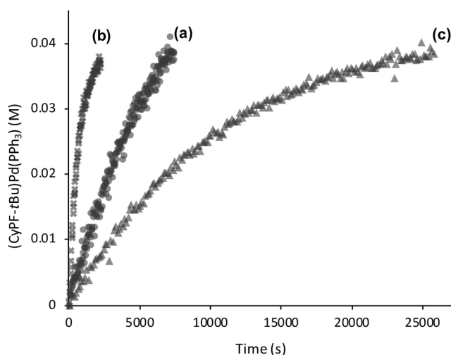
Figure 4. Comparison of rates of product formation for the reaction of arylpalladium(II) complexes 4 and 5 . a) 4 (39.3 mM) with KOH (10 equiv), hydrazine monohydrate (10 equiv), and PPh 3 (2 equiv); b) 5 (39.3 mM) with anhydrous hydrazine (10 equiv) and PPh 3 (2 equiv); c) 5 (39.3 mM) with hydrazine monohydrate (10 equiv) and PPh 3 (2 equiv) in 600 μL of [D 8 ]THF at 35 °C.
