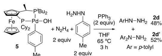
Scheme 6. Competition experiment between hydrazine and p -tolyl hydrazine with aryl hydroxide complex 5 .
