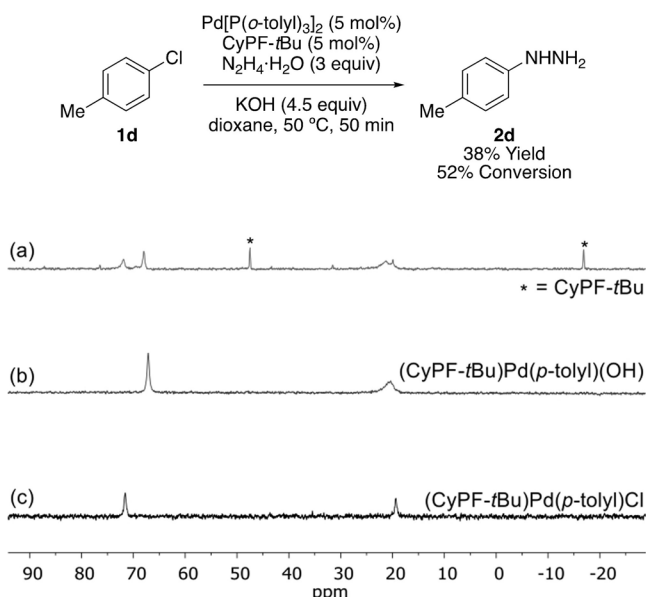
Scheme 1. Determination of catalyst resting state by analyzing the catalytic reaction at partial conversion by 31 P NMR spectroscopy. a) 31 P NMR spectrum of catalytic reaction analyzed at 52% conversion. b) 31 P NMR spectrum of (CyPF-tBu)Pd(p-tolyl)(OH) ( 5 ) in 1,4-dioxane. c) 31 P NMR spectrum of (CyPF-tBu)Pd(p-tolyl)Cl ( 4 ) in 1,4-dioxane.
