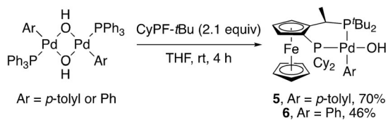
Scheme 2. Synthesis of palladium aryl hydroxide complexes 5 and 6 .
