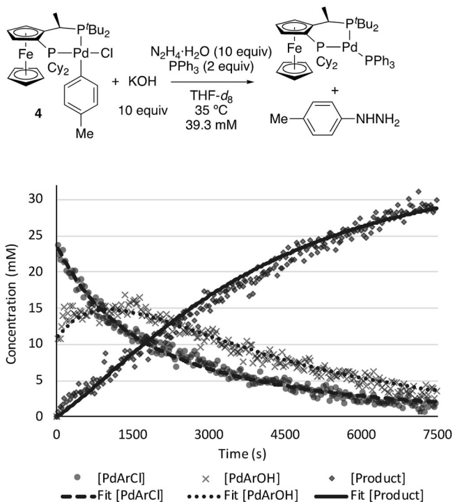
Figure 3. Time course of reaction between (CyPF- t Bu)Pd( p -tolyl)Cl ( 4 ), hydrazine monohydrate, and KOH monitored by ^{31}\text{P} NMR spectroscopy with \text{PMe}_3 as an internal standard and fitted curves obtained from COPASI. The circle trace corresponds to the concentration of 4 , the multiplication sign trace corresponds to the concentration of (CyPF- t Bu)Pd( p -tolyl)(OH) ( 5 ), and the diamond trace corresponds to the concentration of (CyPF- t Bu)Pd( \text{PPh}_3 ).
