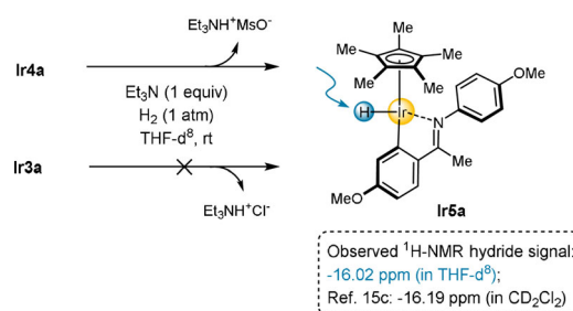
Scheme 6. Stoichiometric iridium hydride formation.
