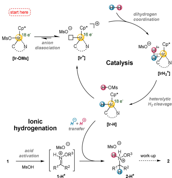
Scheme 7. Suggested reaction mechanism of the ionic iridium-catalyzed oxime hydrogenation.
