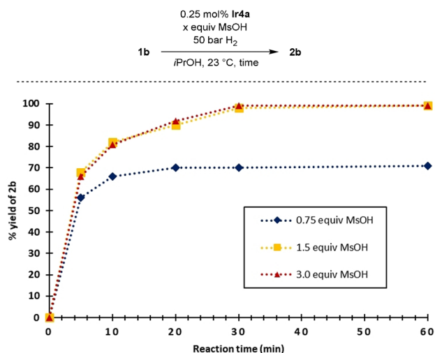
Figure 2. Influence of the acid concentration in the reaction rate. Conditions: 0.3 mmol 1a , 0.23/0.45/0.90 mmol MsOH, 0.25 mol % Ir4a , 50 bar H 2 in i PrOH (0.3 mL) at 23 °C; yield of 2b determined by 1 H NMR using 1,3,5-trimethoxybenzene as internal standard, being equal to the conversion of 1b .
