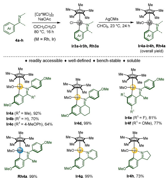
Scheme 3. General synthesis of the cyclometalated \text{Cp}^*\text{M}^{\text{III}} complexes ( \text{M} = \text{Rh}, \text{Ir} ) used for this study. Overall isolated yields are shown for each complex.
