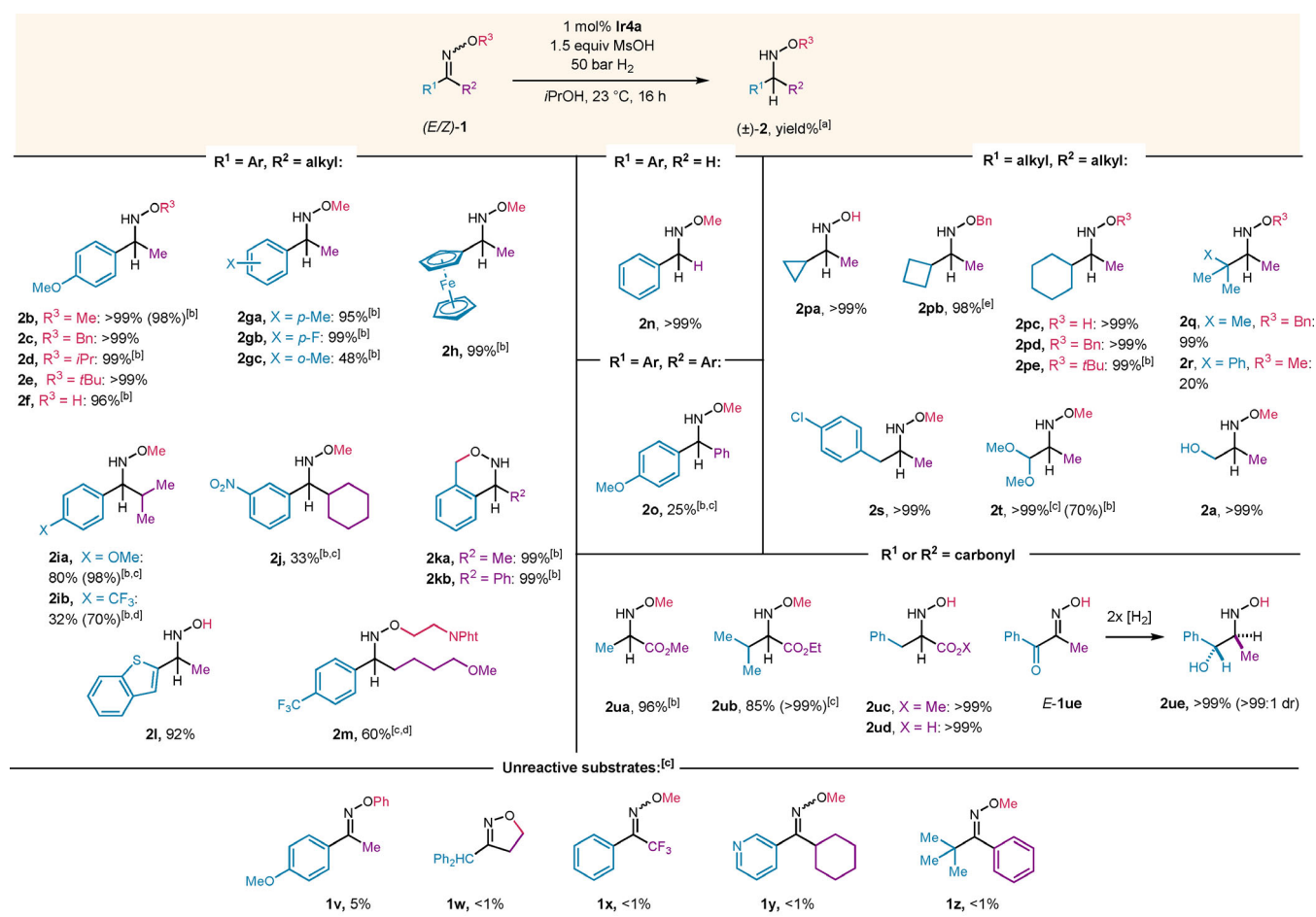
Scheme 4. Substrate scope of the hydrogenation process. Reaction conditions: 0.30 mmol 1 , 0.45 mmol MsOH, 3 \mu\text{mol} Ir4a in i PrOH (0.3 mL) at 23 °C for 16 h. [a] Yields determined by ^1\text{H} NMR using 1,3,5-trimethoxybenzene as internal standard; in all entries the yield equals the conversion of the oxime starting material. [b] isolated yield. [c] in MeOH. [d] with triflic acid. [e] The crude product was N-benzoylated prior to isolation.
