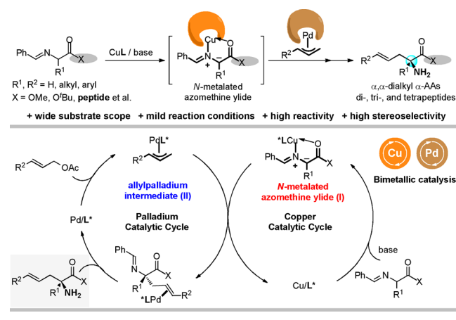
Scheme 1. Bimetallic Catalysis for Stereoselective Modification of Amino Acids and Peptides
