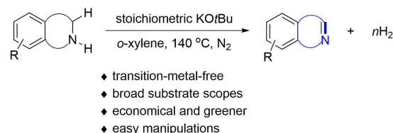
Scheme 1. Acceptorless dehydrogenation of N-heterocycles.
