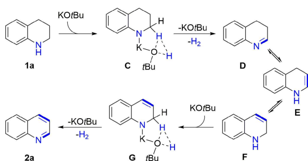
Scheme 3. Proposed mechanism.
