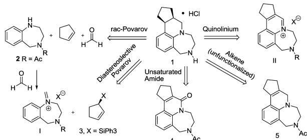
Scheme 1. Retrosynthetic Routes to Vabicaserin ( 1 )
